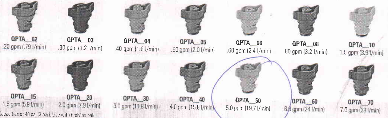
Capacities at 40 psi (3 bar). Use with ProMax ball.
