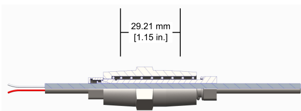
Figure 16: Dimensions
