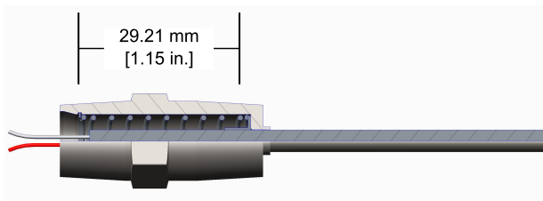
Figure 12: Dimensions
