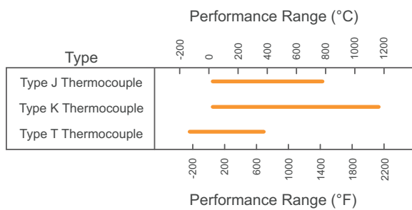
Figure 4: Thermocouple Temperature Ranges
