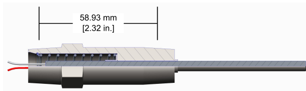
Figure 11: Dimensions
