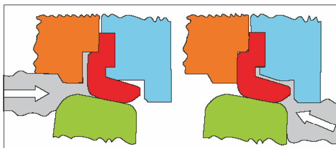
Flexible PTFE Seat
