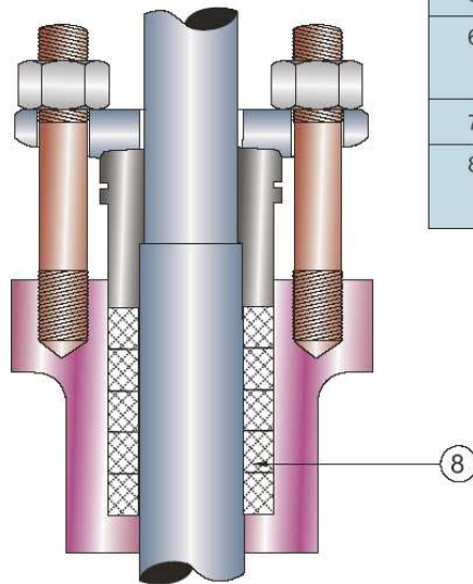
Single Grafoil Packing
