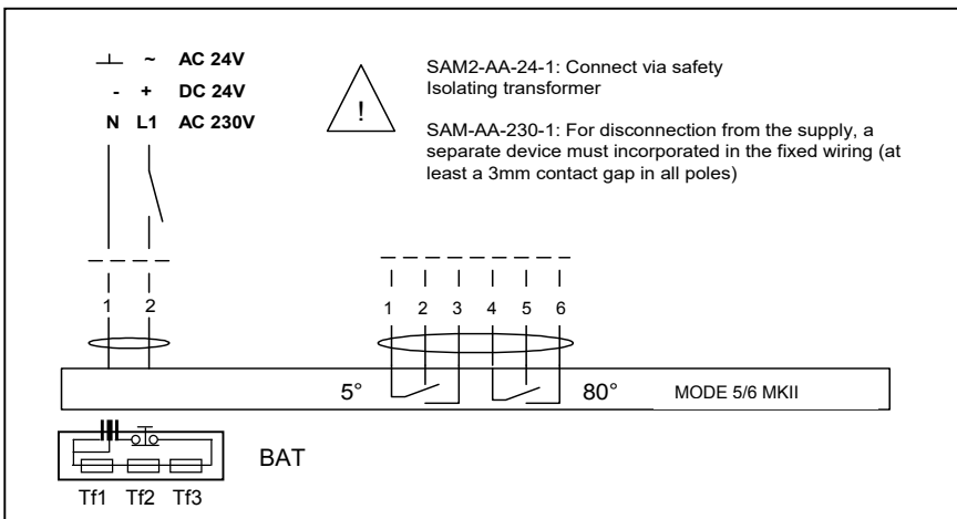
Wiring Diagram
