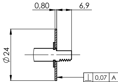
(Shaft detail)
