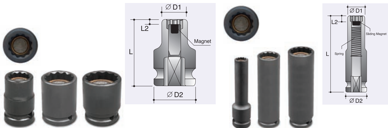
12-Point Sockets
