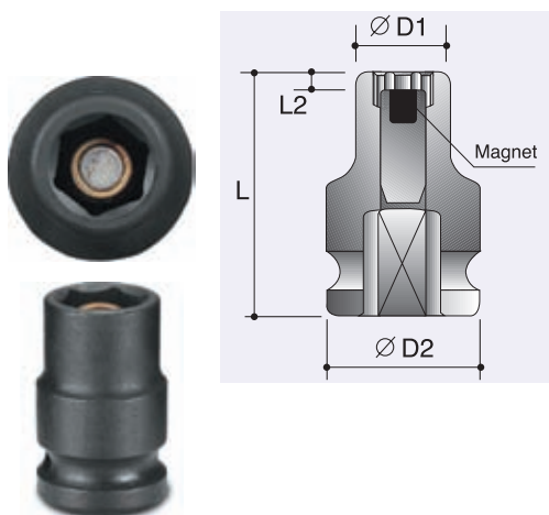
6-Point Sockets
