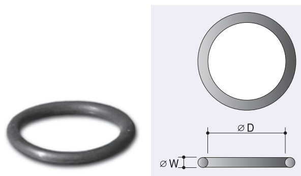
O-Ring
