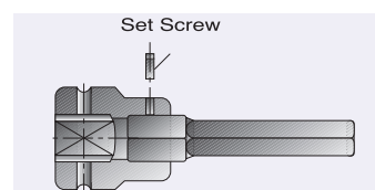
Hex Drivers
