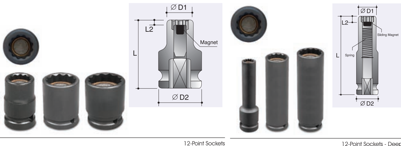
12-Point Sockets
