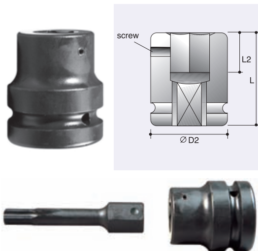
Bit Holders - Set Screw
