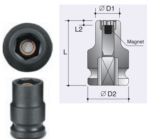
6-Point Sockets
