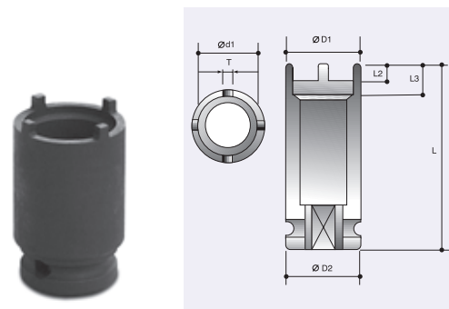
"KM" Type Axial Nut Sockets
