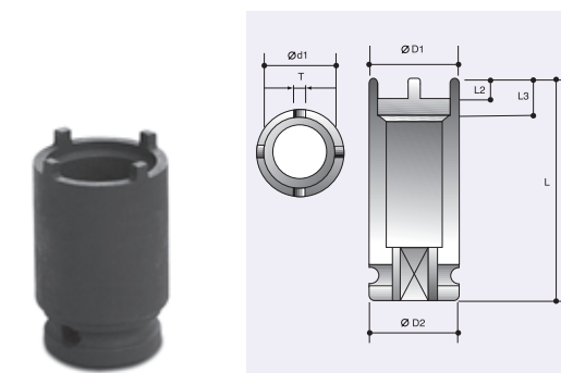
"GU" Type Axial Nut Sockets
