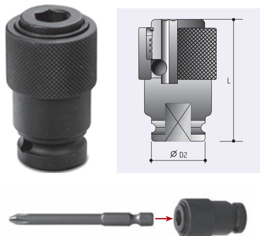
Quick Releasing Chucks
